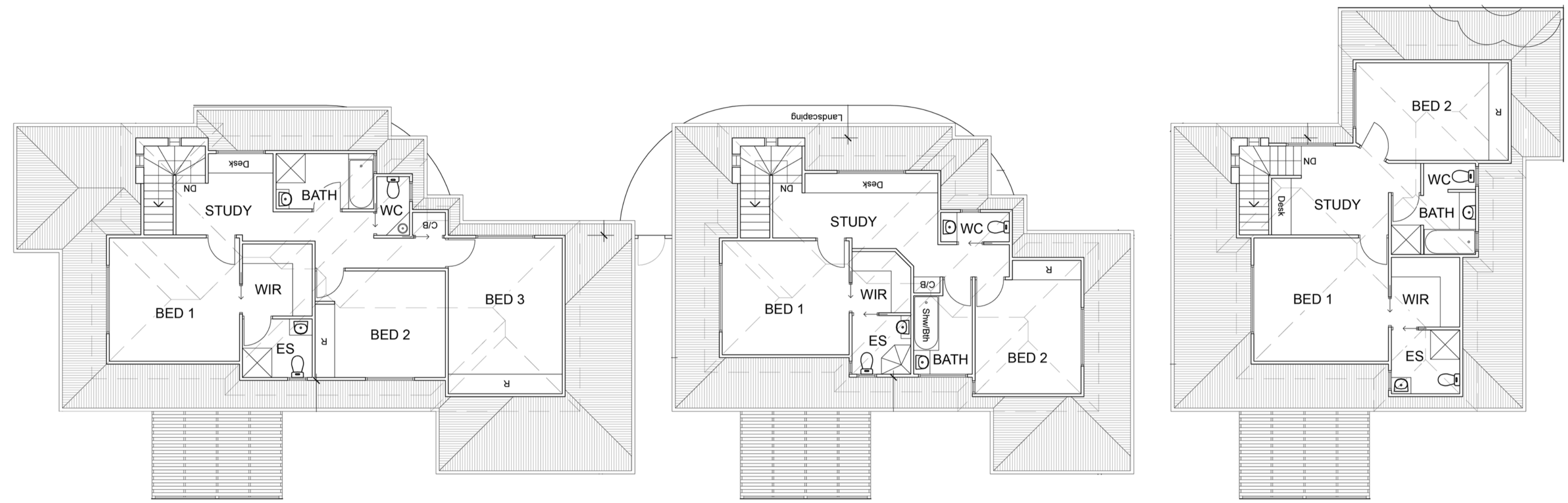
UPPER FLOOR PLAN
